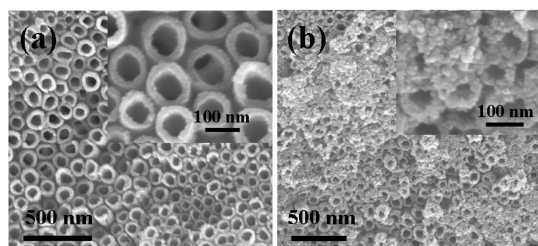
FIGURE 2. FESEM images of (a) CdS/TNTAs and (b) sonication-CdS/TNTAs.
